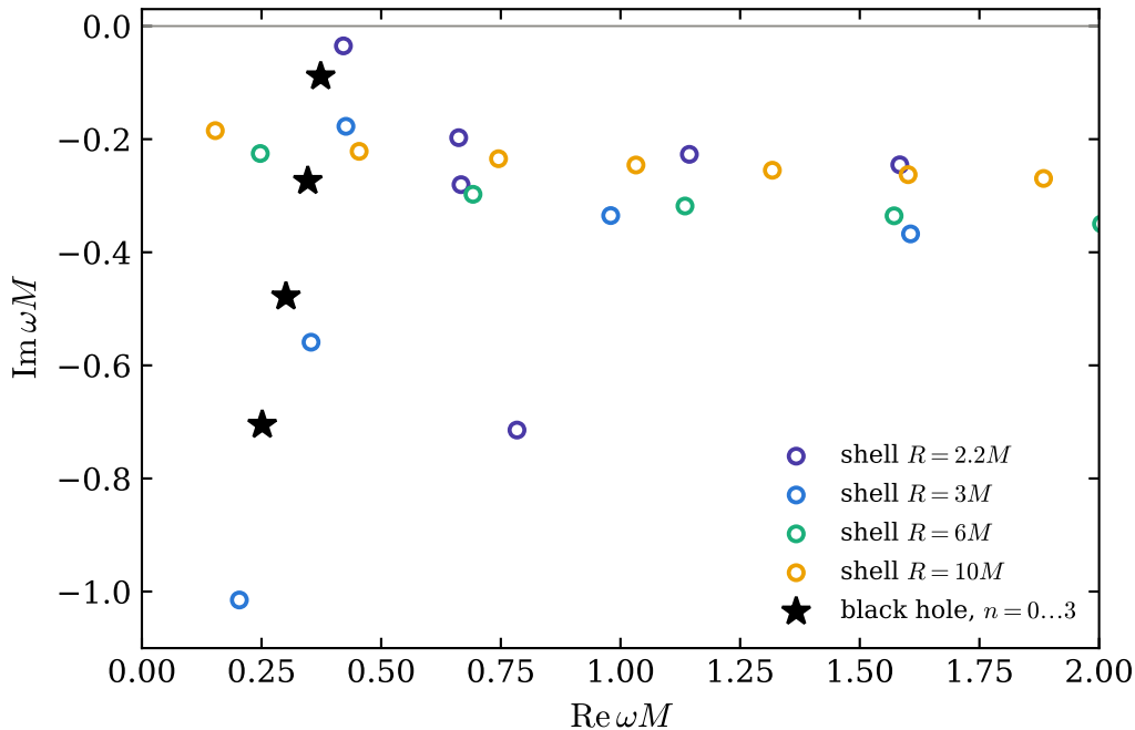
Odd-parity QNMs, \ell = 2 : the shell does not ring like a black hole
